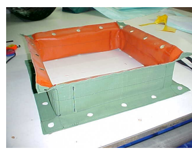
Expansion Joint with Inner Silicone High Temp Cloth
